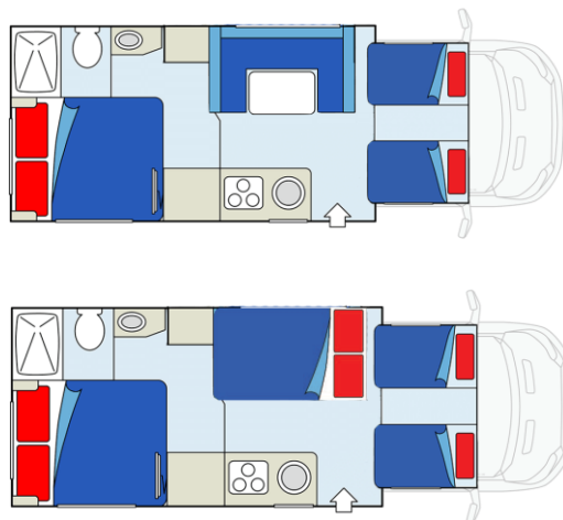
Compact Motorhome MHC
